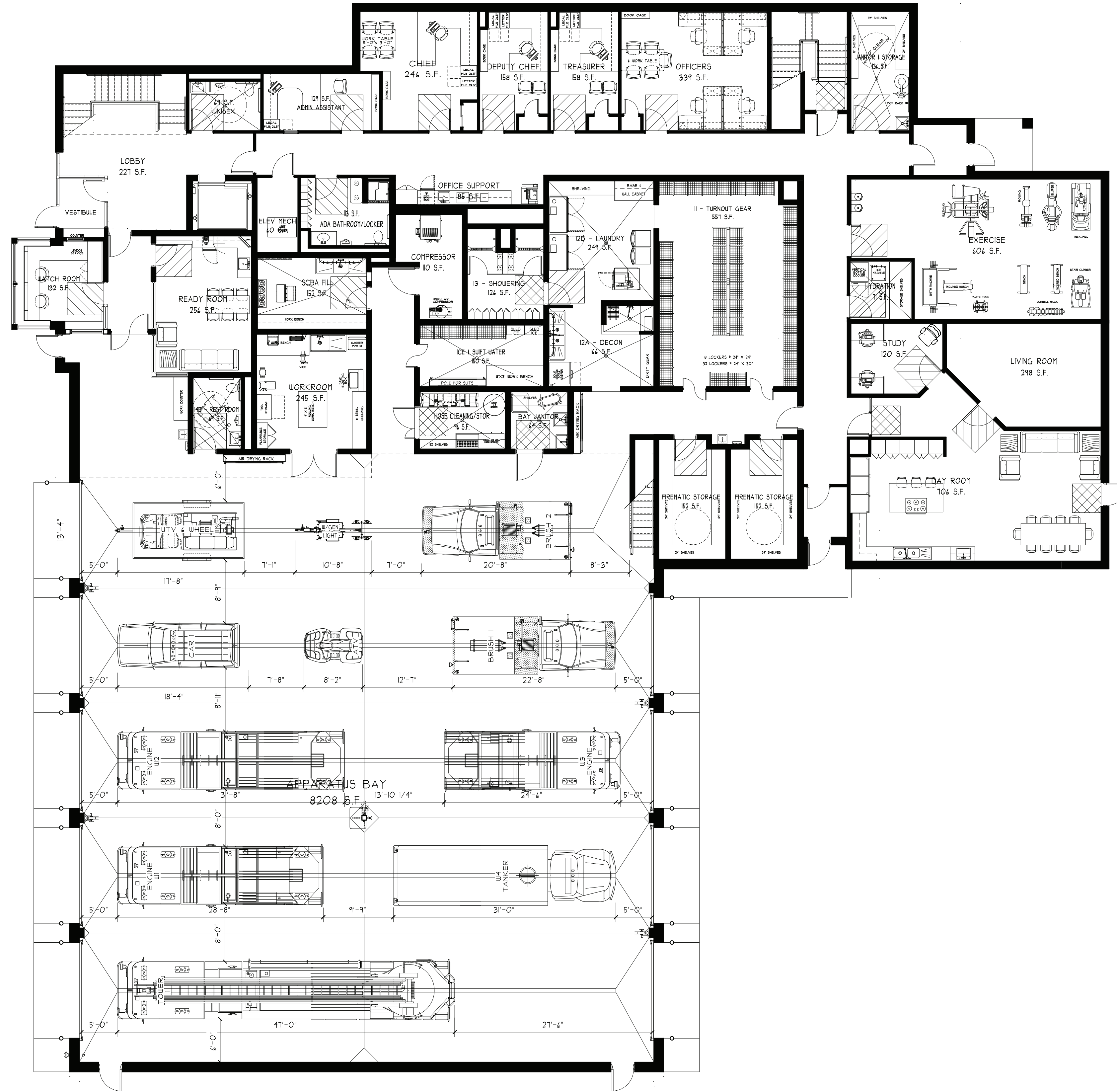
FIRST FLOOR 1/8" = 1'-0"
